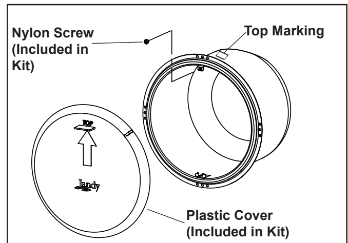
Figure 7. Plastic Niche Cover and Nylon Screw for Stainless Steel Niche
