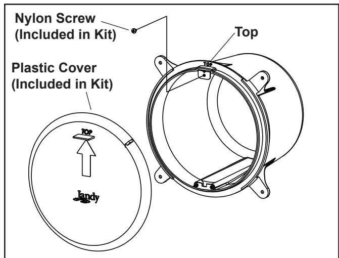
Figure 4. Plastic Niche Cover and Nylon Screw for Plastic Niche
