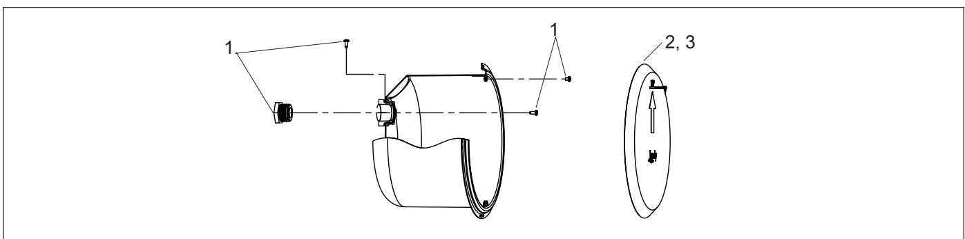
Figure 9. Stainless Steel Pool and Spa Niche (SSNICLRG1X and SSNICSM1X) Exploded View
