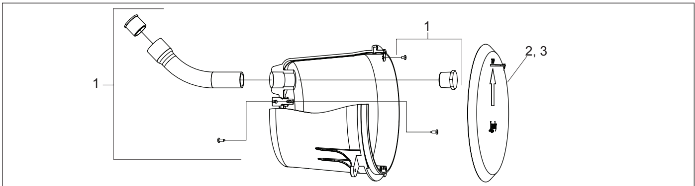
Figure 8. Plastic Pool and Spa Niche (PLNICLRG and PLNICSM) Exploded View
